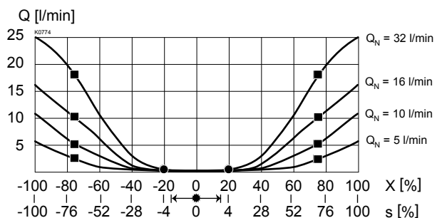
Q = f(s, x) Volume flow-signal-characteristics ( \Delta p = 10 \text{ bar} ) [Type: ADB-V] ( s corresponds to preset value signal and x corresponds to spool stroke)
