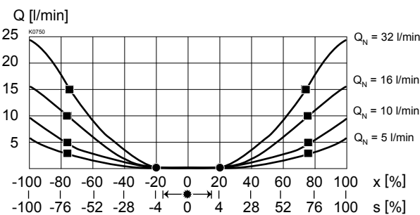
Q = f(s, x) Volume flow-signal-characteristics ( \Delta p = 10 \text{ bar} ) [Type: ACB-S] ( s corresponds to preset value signal and x corresponds to spool stroke)
